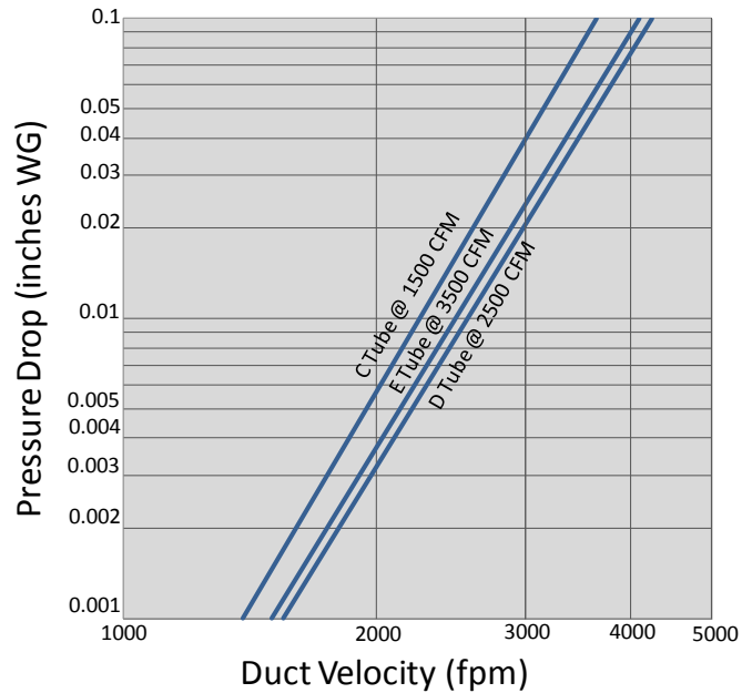
Pressure Drop vs. Duct Velocity
